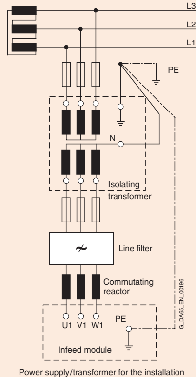
Single-pole circuit diagram with IT supply system and isolating transformer
