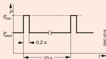
Peak output duty cycle with preloading condition
