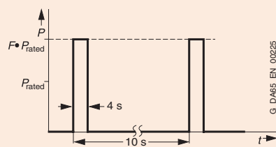
Peak output duty cycle with preloading condition
