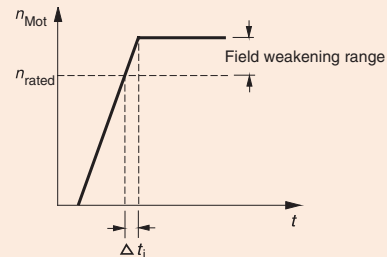
Example of motor speed and motor torque in a time segment \Delta t_i
