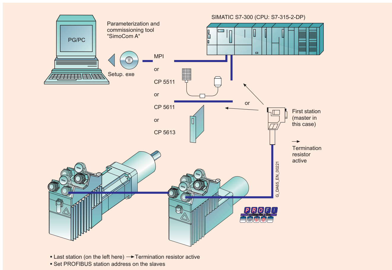
Example of online operation via PROFIBUS: "SimoCom A" ↔ 2 drives
