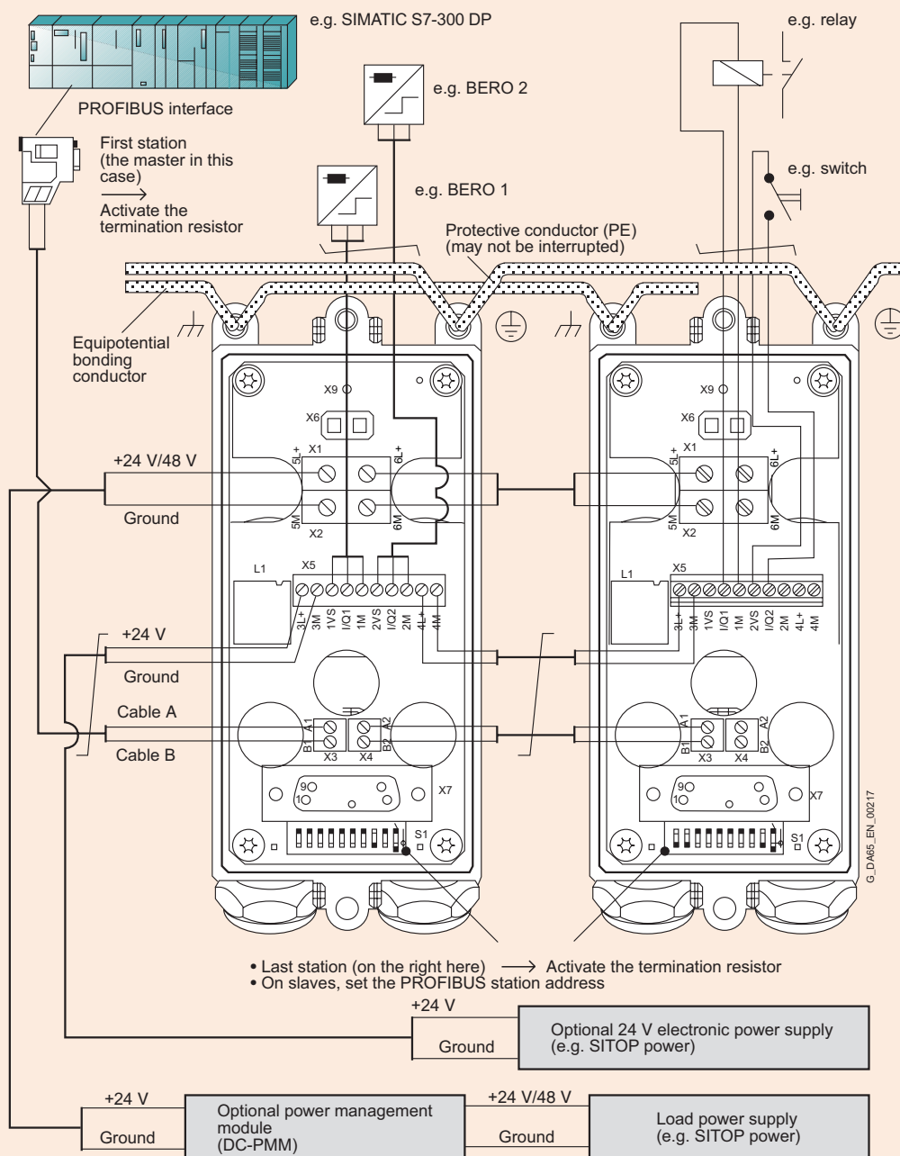
Connection and wiring overview (example with additional electronics supply)
