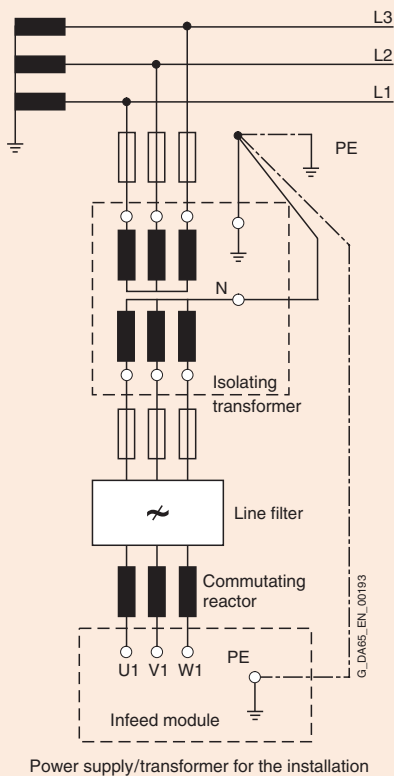
TT supply system with grounded star point and isolating transformer
