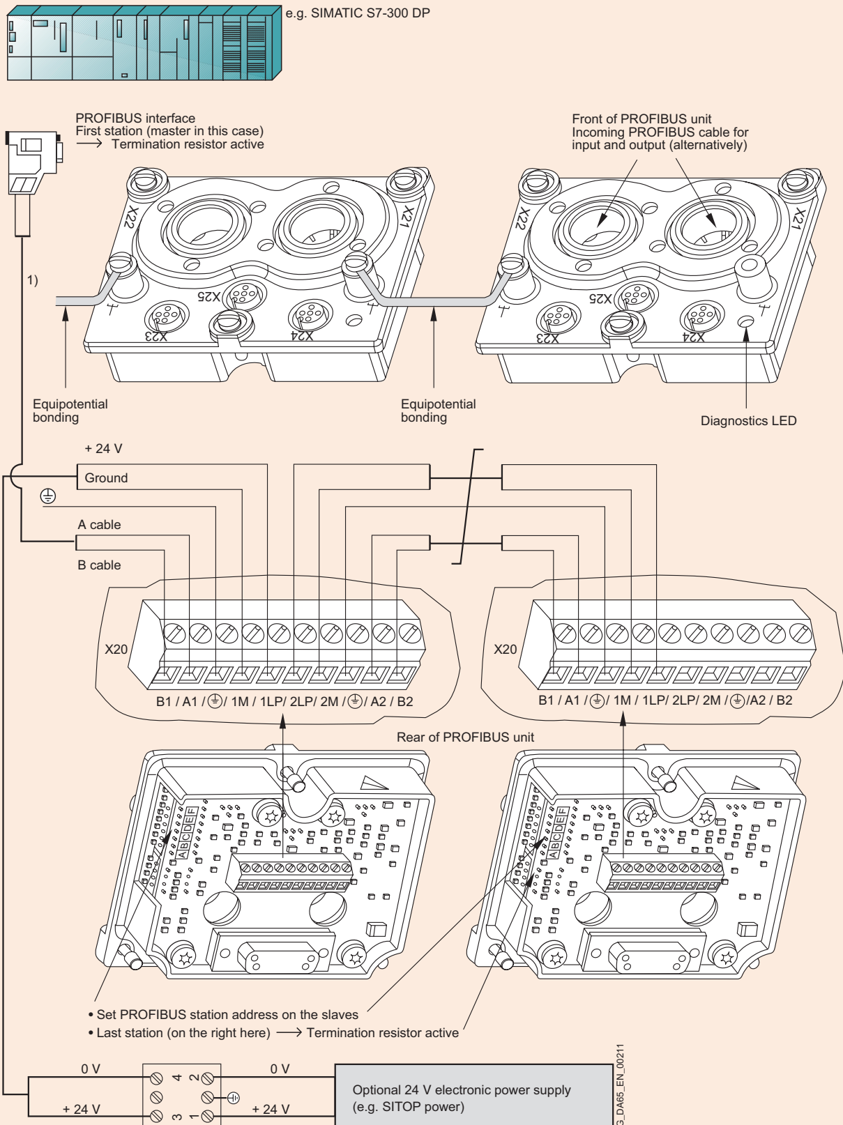
Connection and wiring overview with PROFIBUS cable (example with additional electronics supply)
