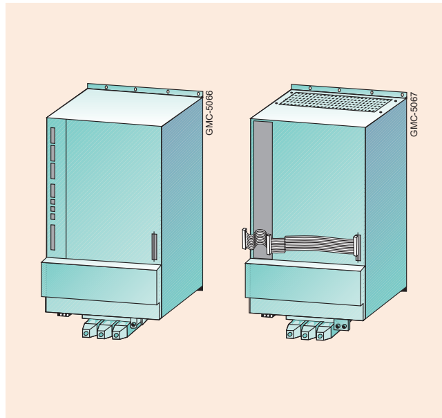
Infeed/regenerative feedback module, internal cooling (left) Power module, internal cooling with internal fan (right)
