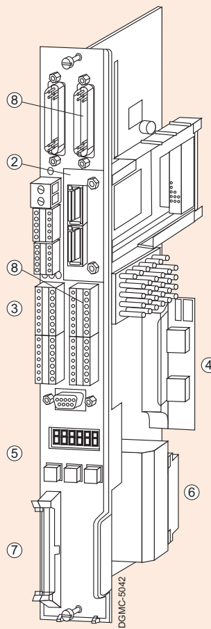
Control unit for resolver
