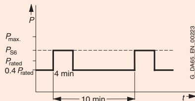
S6 duty cycle with preloading condition
