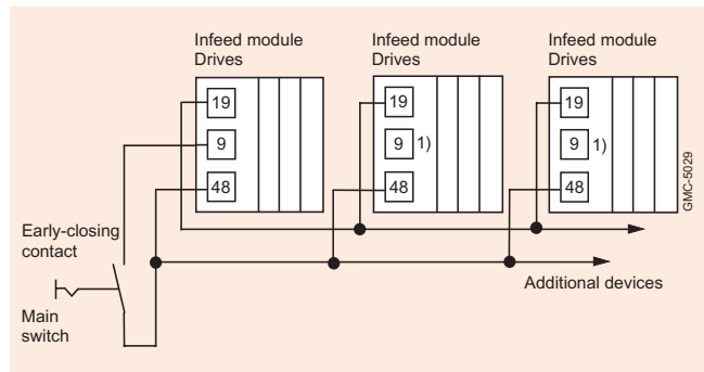
Connection diagram
