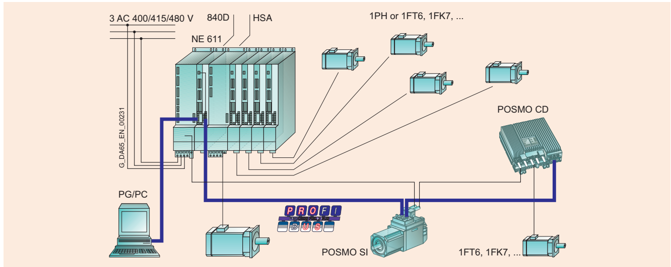
Mixed mode with SINUMERIK 840D (master) and SIMODRIVE 611D (NCU 573.2 only)
