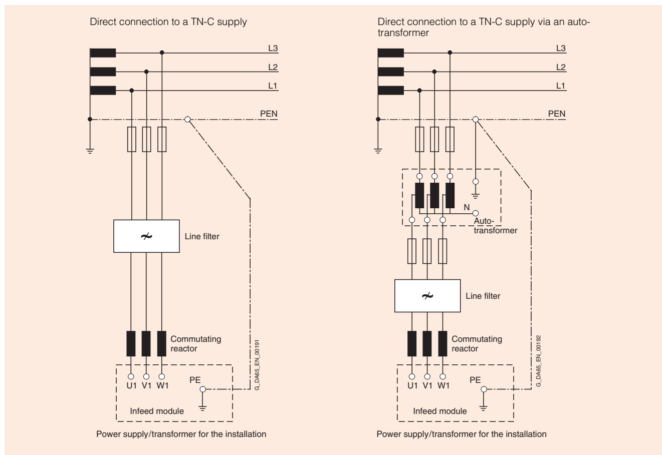
Connection to TN-C supply systems
