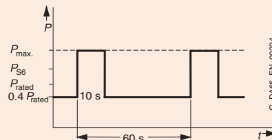
Peak output duty cycle with preloading condition
