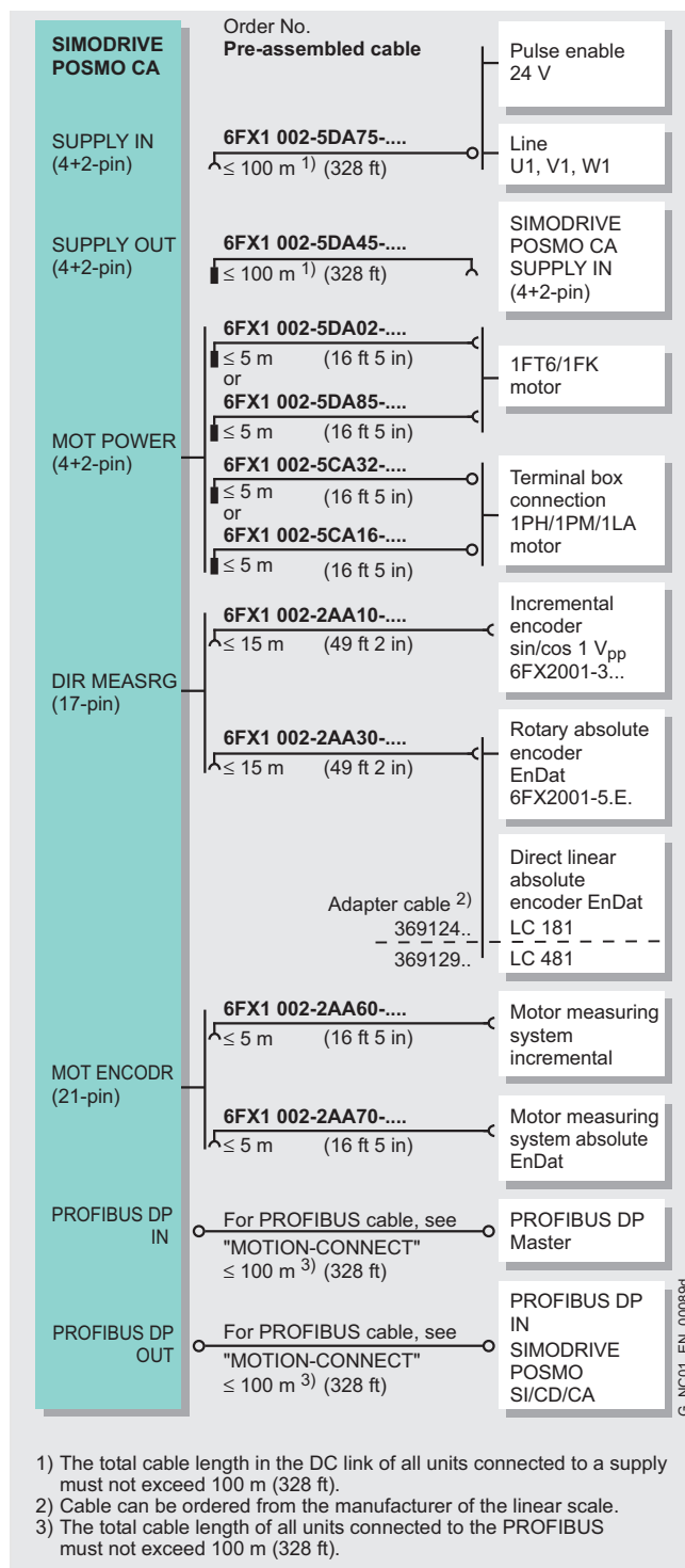
Connection overview for SIMODRIVE POSMO CA
