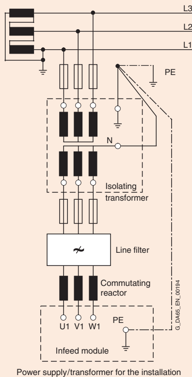
TT supply system with grounded phase and isolating transformer
