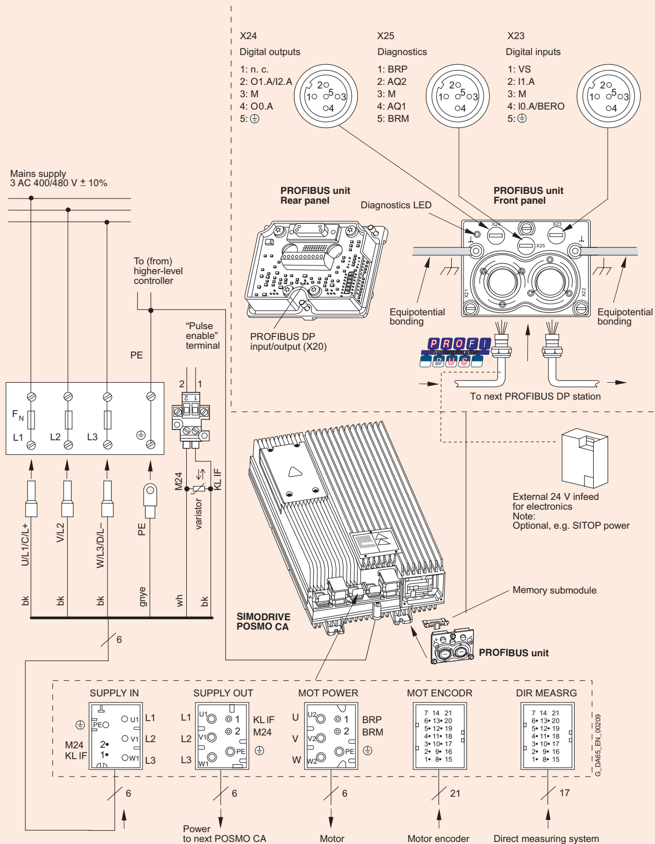
Connection overview for SIMODRIVE POSMO CA
