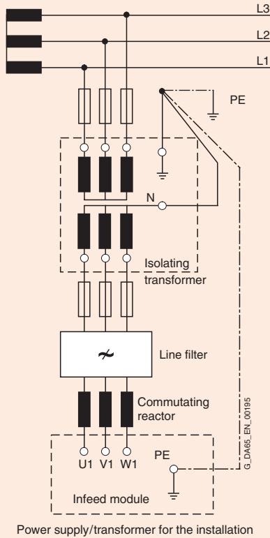
Single-pole circuit diagram with IT supply system and isolating transformer
