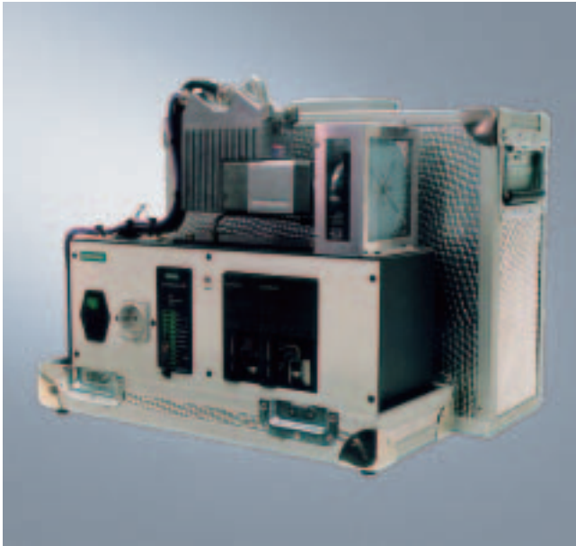
SIMODRIVE POSMO A training case with 1 axis
