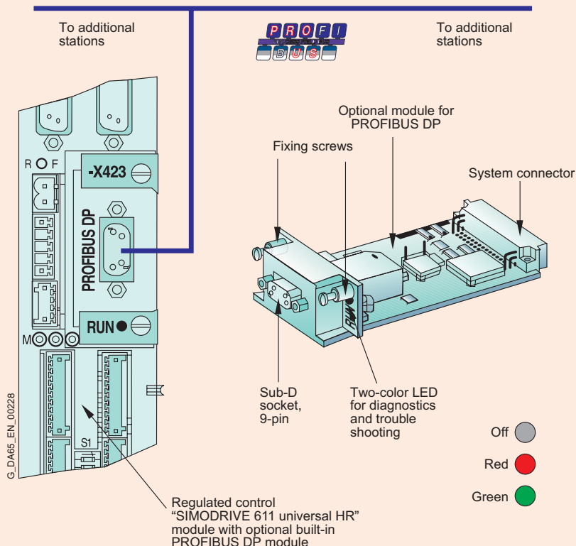
SIMODRIVE 611 universal HR with PROFIBUS DP option module
