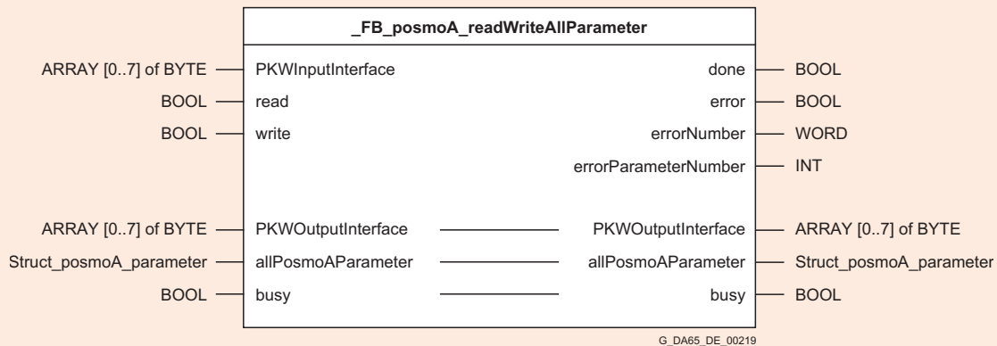
Schematic LAD diagram
