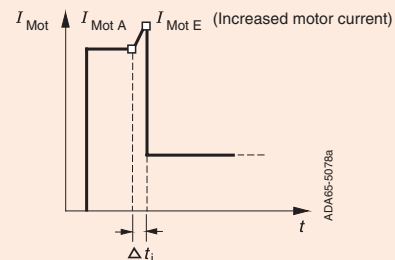
Example of motor speed and motor current in a time segment \Delta t_i
