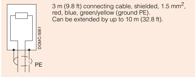
Connection of an external 0.3 kW/25 kW pulsed resistor
