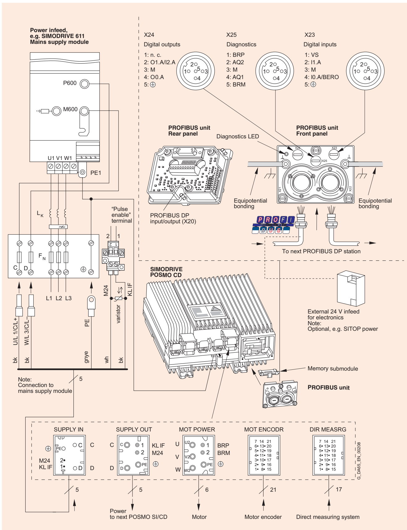
Connection overview for SIMODRIVE POSMO CD
