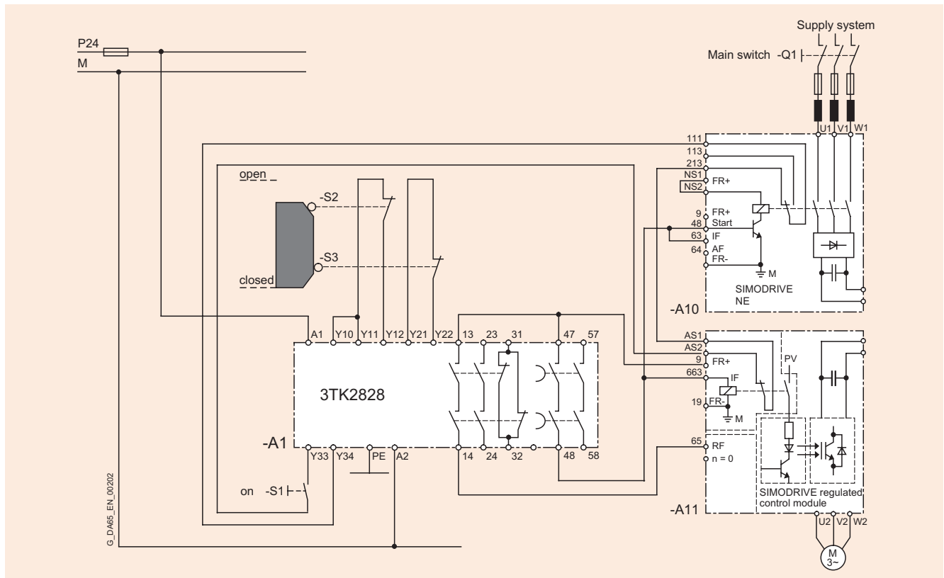
"Safe standstill" with SIMODRIVE with an unlocked protective door, with safety combination, stop category 1, category 3 to EN 954-1
