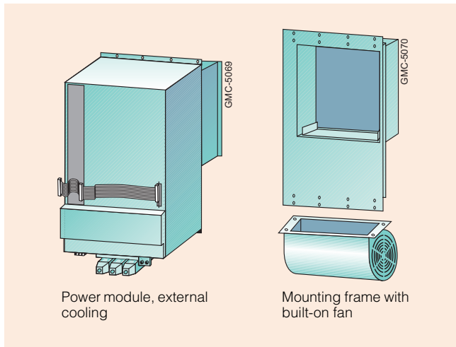
External cooling of the power module and mounting frame with built-on fan
